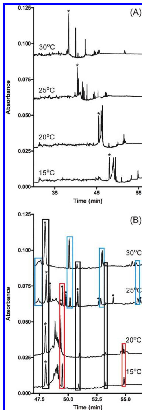
Figure 3. Thermal dissociation studies of the Dam1 complex. (A) CIEF separations of 500 \mu\text{g/mL} Dam1 complex at different separation temperatures using a 100 \mu\text{m} HPC coated capillary. The peaks marked with (*) were used as a mobilization marker for viscosity corrections. (B) The same CIEF separations from (A) viscosity corrected and expanded in the region of Dam1 complex peaks. Potential subcomplex peaks were marked with (●) in the 25 °C separation. Peaks that were common to specific separation temperatures were enclosed with a box, marking individual proteins (blue), subcomplexes (red), and potentially individual proteins, system peaks, or impurities (black).
