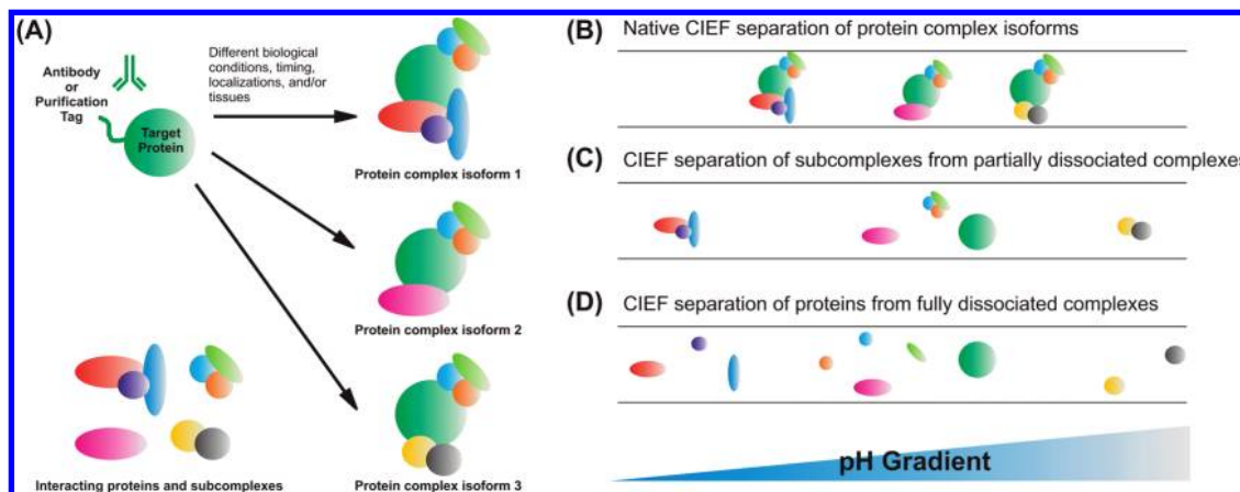
Figure 1. Schematic of protein complex isoforms and subcomplexes and their CIEF separations. (A) The composition of protein complexes are often elucidated through purification of a target protein, and all proteins associated with it, using an antibody or purification tag. The purification creates a heterogeneous mixture of protein complexes, called protein complex isoforms. Three examples are shown here. Each protein complex isoform can be composed of different proteins or subcomplexes depending on its specific function under certain biological condition. (B) A theoretical native CIEF separation of the three protein complex isoforms. Although many proteins are similar in each protein complex isoform, the proteins or subcomplexes which are different shift the isoelectric point of the protein complex isoform. This inherent pI shift allows for separation within the pH gradient generated using CIEF. (C) Dissociated protein complexes are known to maintain more thermodynamically stable subcomplexes. These subcomplexes can also be separated based on their isoelectric points using native CIEF. (D) A traditional CIEF separation of individual proteins from fully dissociated protein complexes isoforms and subcomplexes using denaturants or thermal dissociation. Note that the pIs of the separated proteins contribute, likely as a weighted average, to the pIs of the subcomplexes they are associated with in the separation above. Likewise, comparison of the subcomplex separation in (B) to the complex isoform separation in (A) illustrates how the pIs of proteins and subcomplexes contribute to the pI of the complex isoform.
