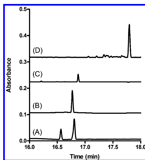
Figure 5. CIEF separations of 25 \mu\text{g/mL} mTORC1 and 2 with different conditions using a 50 \mu\text{m} PVA coated capillary. (A) Successful separation of mTORC1 and 2 upon immediate analysis with 1.7% w/v pI 3–10 and 2.1% w/v pI 4–6.5 ampholytes. (B) Replicate analysis of mTORC1 and 2 as in (A) after 5 h. (C) Separation of dissociated mTORC1 and 2 as in (A) after storage at 4 °C for one week. (D) Unsuccessful separation of mTORC1 and 2 using only 1.7% w/v pI 3–10 ampholytes.
